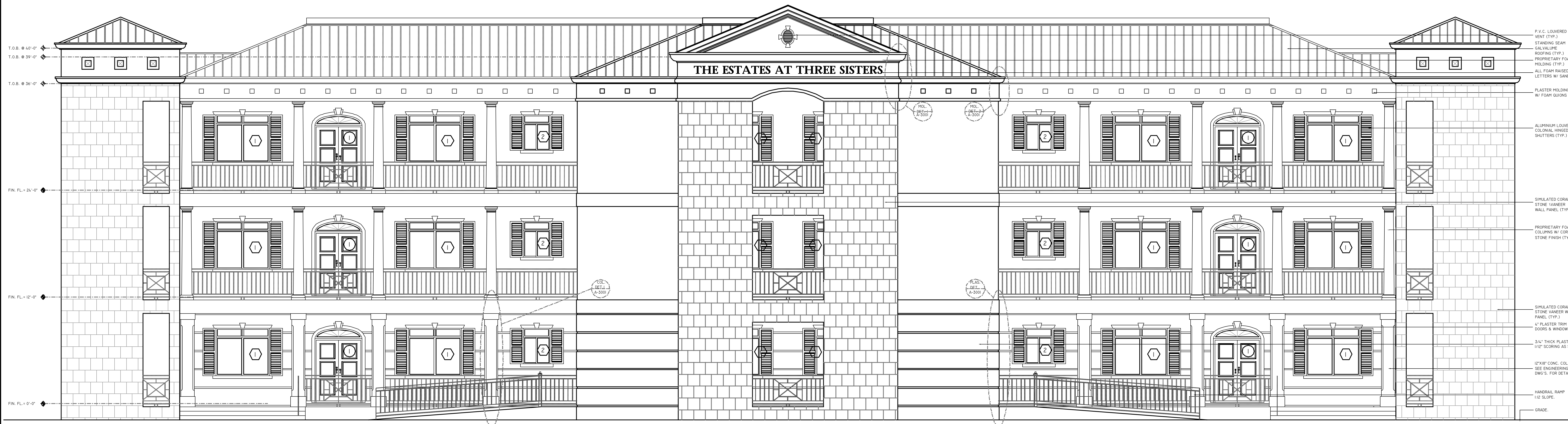
PROPOSED FRONT ELEVATION: SCALE: 1/4"=1'-0"
